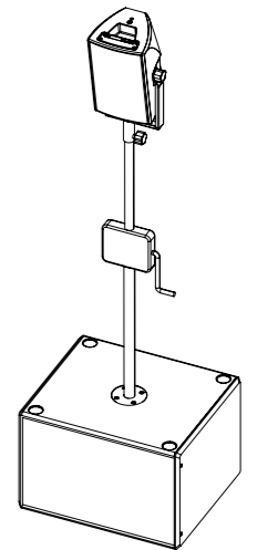
E6 with Z5377 E6 Swivel bracket Z5034 Stand adapter M10 Z5013 Loudspeaker stand winder M20
