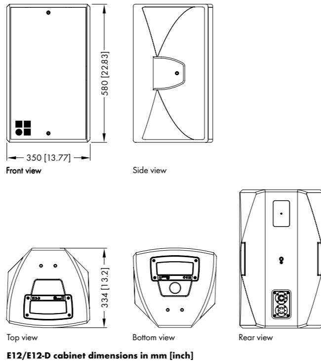
E12/E12-D cabinet dimensions in mm [inch]
